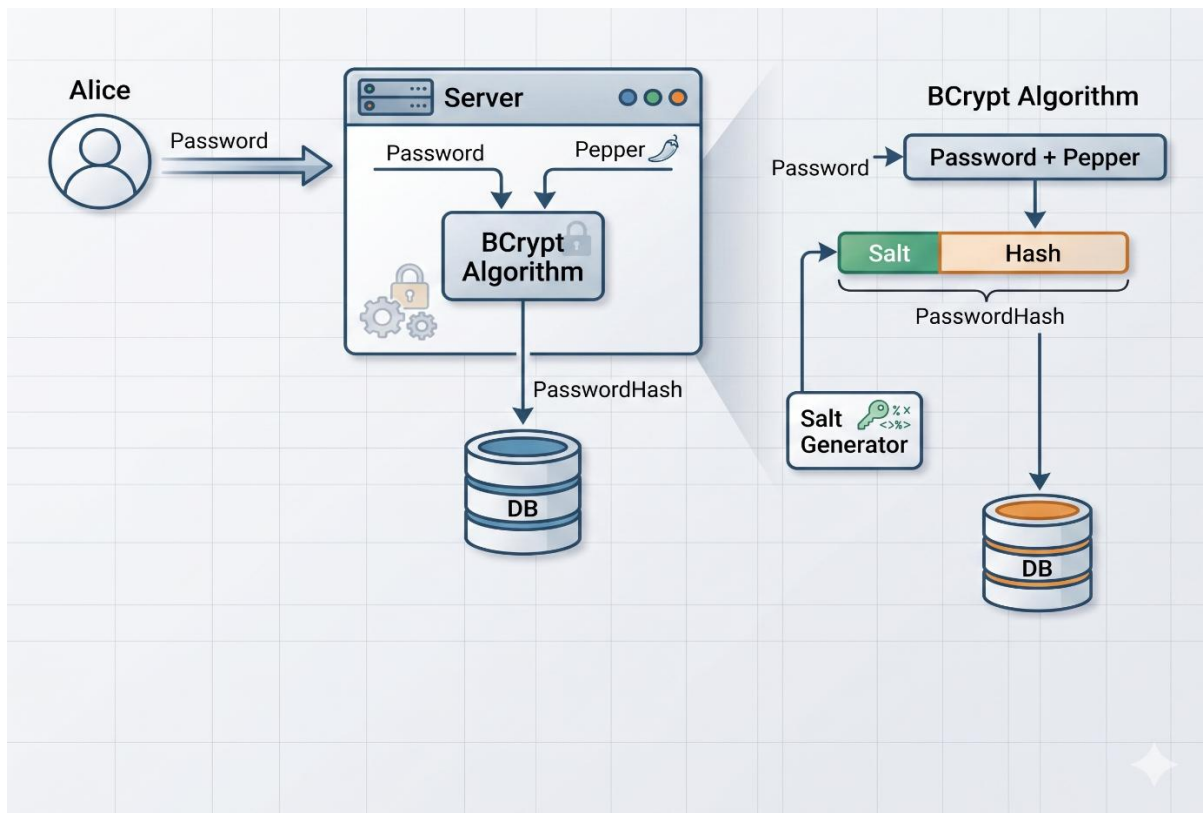
Figure 3-2: BCrypt Algorithm Process
