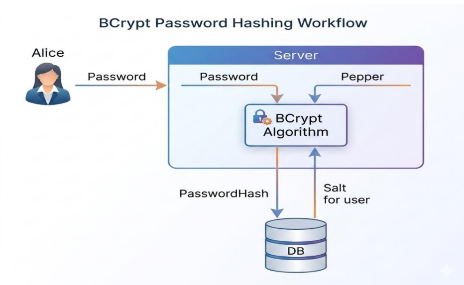
Figure 3-3: Identification/ Password Validating
